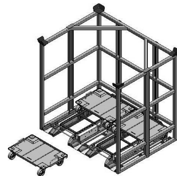
Item no. 201537 for BOZ 630 x 430 mm see chapter TROLLEYS BOZ
